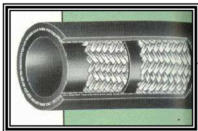
Air Brake Hoses (SAE J1402-unarmoured)
